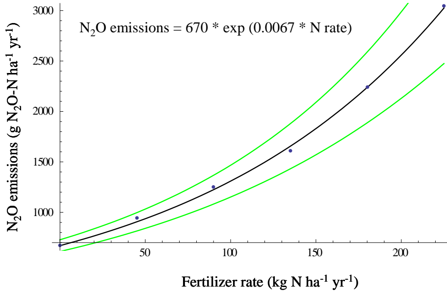
Figure G1. Relationship between N_2O emissions ( g N_2O-N ha^{-1} yr^{-1} ) and N fertilizer rate ( kg N ha^{-1} yr^{-1} ) for baseline and project N fertilizer rates (black line). Standard errors ( \pm 58 * \exp [0.010 * N \text{ rate}] ) are also shown (green lines). Calculated using Mathematica (v. 8, Wolfram Research Inc., 2011).
