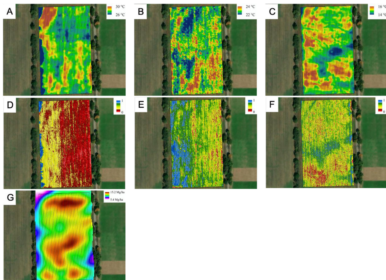
FIGURE 5 Thermal imagery (AirScout, Inc.) at KBS 30-2 in 2017. (a) Thermal image on 16 June, (b) thermal image on 28 June, (c) thermal image on 6 Sept., (d) advanced difference vegetation index on 16 June, (e) advanced difference vegetation index on 28 June, (f) advanced difference vegetation index on 6 Sept., (g) final yield map
