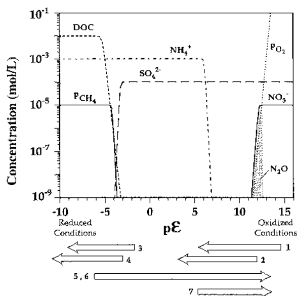
FIG. 1. Predicted thermodynamic equilibrium concentrations of selected electron donors and acceptors as a function of the redox state pE of the environment at pH 7. pE is a measure of the electron activity, which, in turn, is one way to characterize the oxidation state of a system: pE = -\log(e^-) . More-negative values indicate a reducing environment or reaction, while more-positive values indicate oxidizing conditions. The expression " pE " shares a similar origin to pH, which is a common measure of the activity of hydrogen ions in a system: pH = -\log(H^+) . DOC = dissolved organic carbon; P_{O_2} and P_{CH_4} are partial pressures. Concentration lines are based on the following reactions from Table 1: O_2 = aerobic respiration (1) in system open to atmosphere; NO_3^- = denitrification to N_2 (2) with [NO_3^-] + 2 \times [N_2] = 10^{-3} mol/L; SO_4^{2-} = sulfate reduction (3) with [SO_4^{2-}] + [HS^-] = 10^{-4} mol/L; CH_4 = product of methane fermentation (4) with [CH_4] + [CO_2] = 10^{-5} mol/L; NH_4^+ = nitrification (7) with [NH_4^+] + [NO_3^-] = 10^{-3} mol/L; DOC = oxidation of succinate to CO_2 with \Sigma C = 10^{-2} mol/L. Numbered arrows indicate approximate regions for these reactions, and for sulfide oxidation (5) and methane oxidation (6) in natural environments. The shaded area indicates the approximate region for transient N_2O accumulation during denitrification (Tiedje 1988). These ideal predictions may not always be realized in natural environments due to nonequilibrium conditions or variations in concentrations of reactants and products. Adapted in part from Stumm and Morgan (1981).
