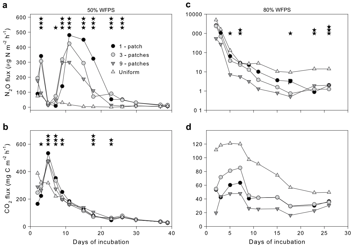
Fig. 3. Litter aggregation and soil moisture content influence on \text{CO}_2 and \text{N}_2\text{O} flux. (a,c) \text{N}_2\text{O} flux from litter aggregation as influenced by 50% and 80% WFPS, respectively; (b,d) \text{CO}_2 flux from litter aggregation as influenced by 50% and 80% WFPS, respectively. ANOVA results comparing the mean of the aggregated litter treatments to the uniformly distributed litter are presented across the top of each graph. Statistical significance at * P < 0.05 , ** P < 0.01 , and *** P < 0.001 for the contrasts. In (d) the repeated measures ANOVA indicates that the \text{CO}_2 flux was significantly greater ( P < 0.05 ) in the uniform distribution than the mean of the aggregated litter throughout the entire incubation. Note the differences in scales between the left and right panels.
