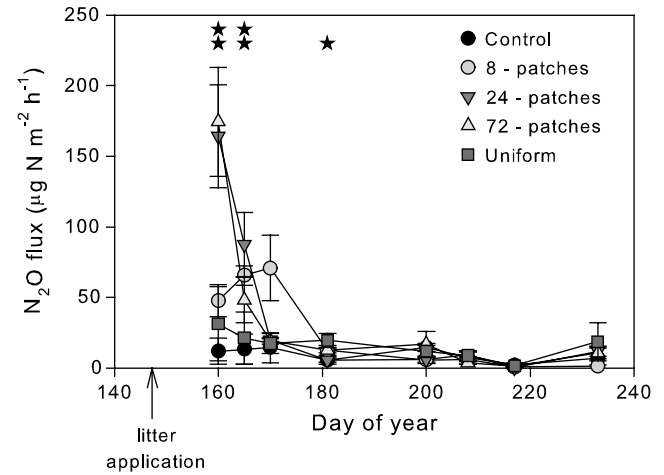
Fig. 5. Nitrous oxide flux by day of year (DOY) from litter aggregation with field-grown maize plants in 50-L mesocosms. ANOVA results are presented across the top of the graph. Statistical significance at the *P < 0.05 and **P < 0.01 , for the contrast between aggregated and uniformly distributed litter. The error bars indicate one standard error.
